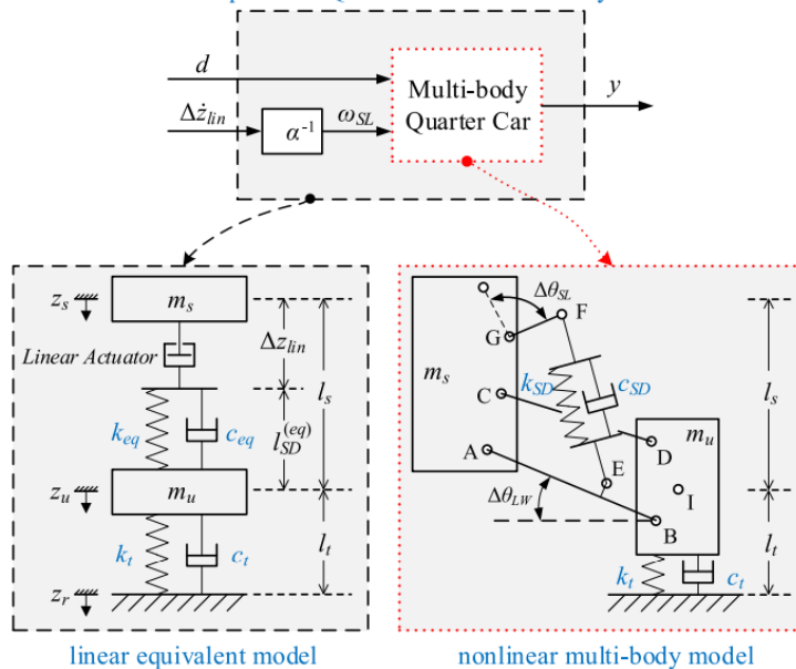
Linear Equivalent Quarter Car for Control Synthesis
